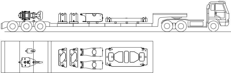
28.2t: Counterweight block + carbody counterweight + hook
